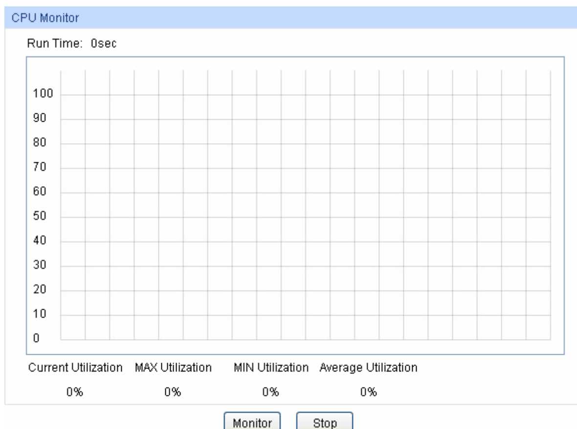
Figure 11-1 CPU Monitor
